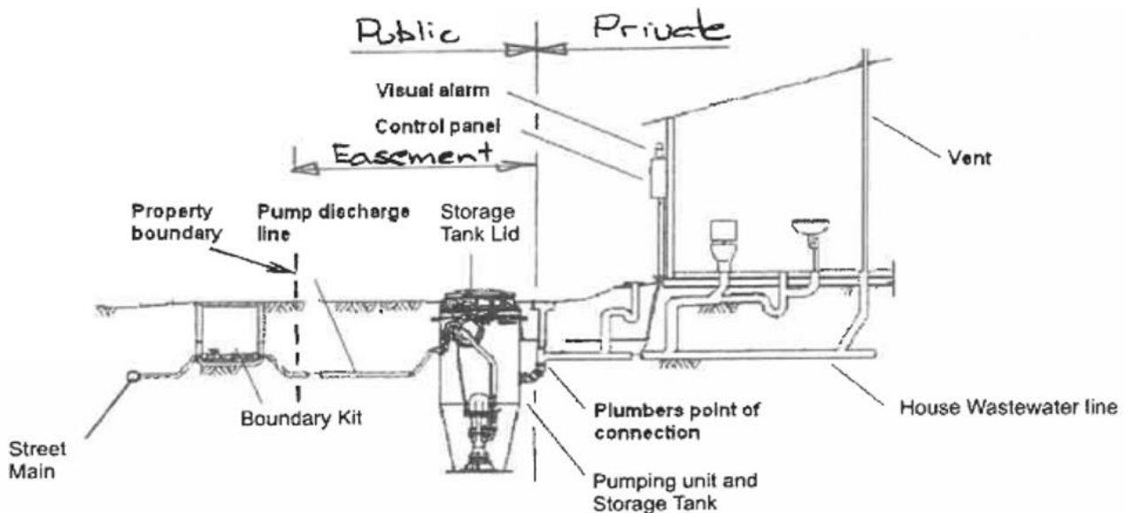
Figure 1- Typical on-property Pressure Wastewater Pumping System
